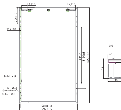
HT60-156P(PD)-F / HT60-156P(PDV)-F
