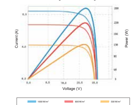
I-V Curves
