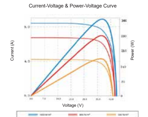
I-V Curves
